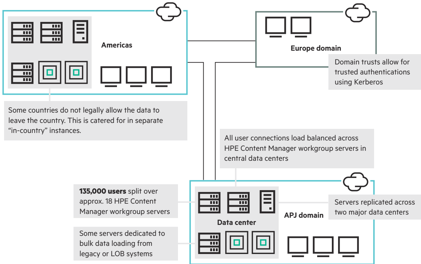
Figure 11: Decentralized implementation example 2
