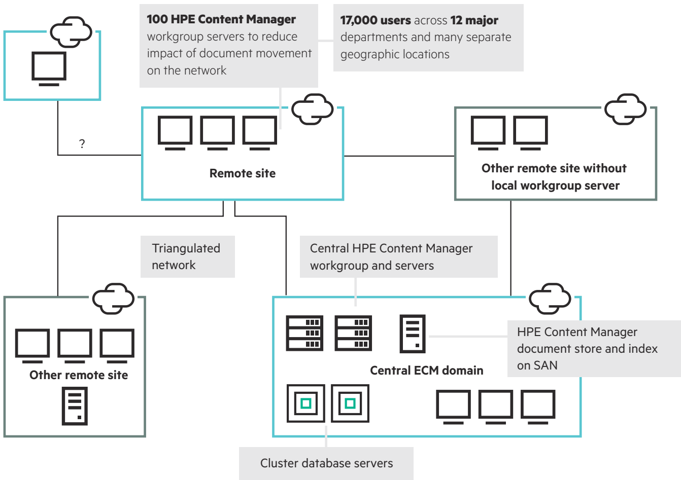
Figure 10: Decentralized implementation example 1
