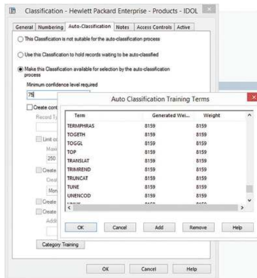
Figure 3: Auto-classification dialogue
